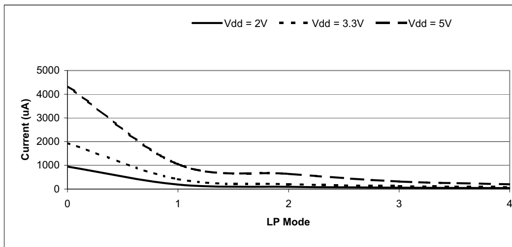
Figure 6-3. Idd Curve
